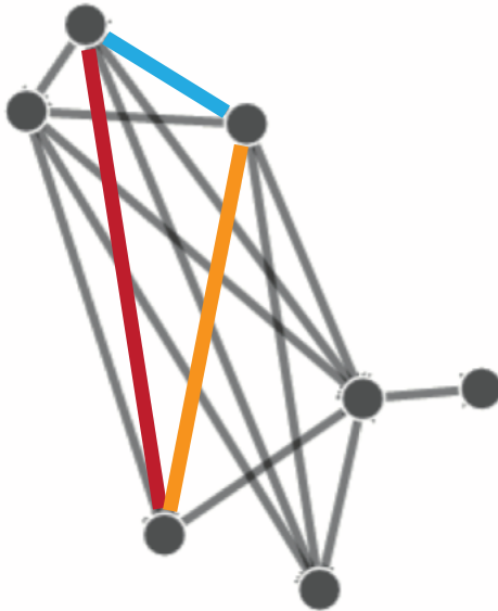
Node-link diagram
